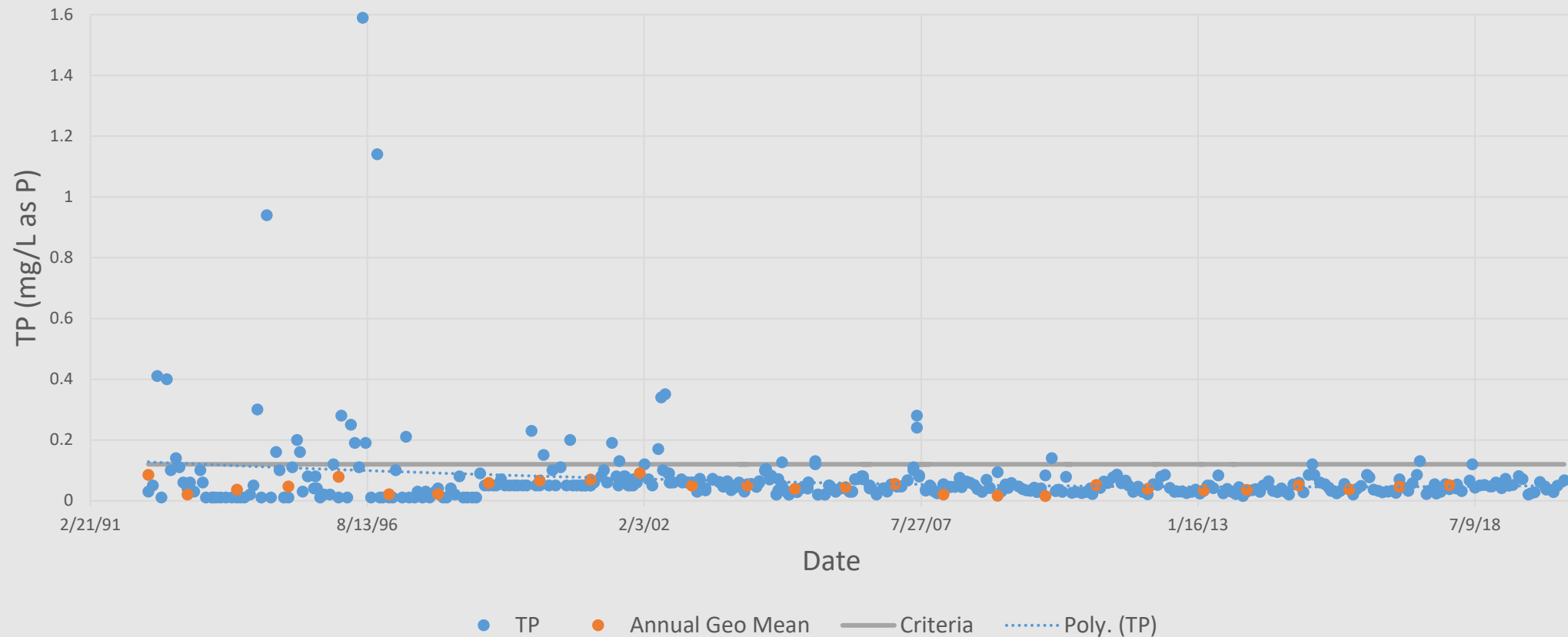
Estero River at Riverwoods (47A-4GR) Total Phosphorus
