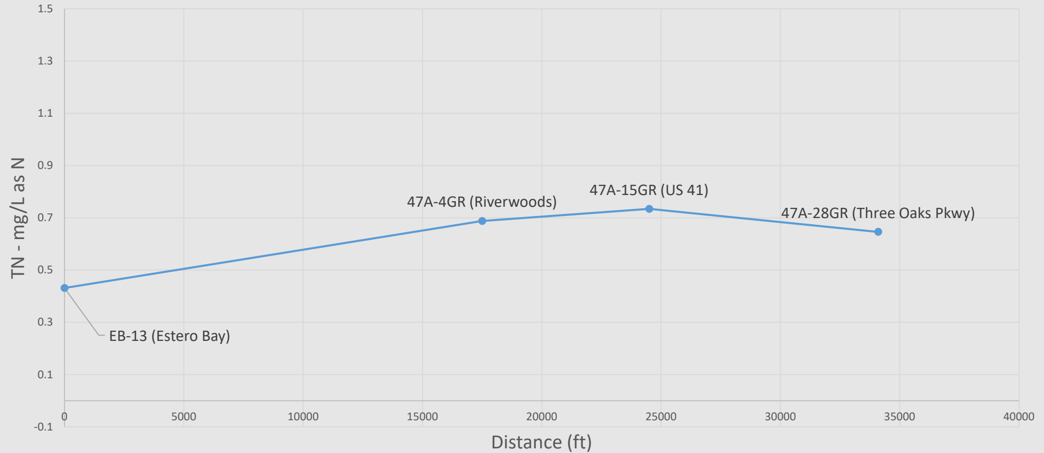
Estero River - Total Nitrogen (TN)
