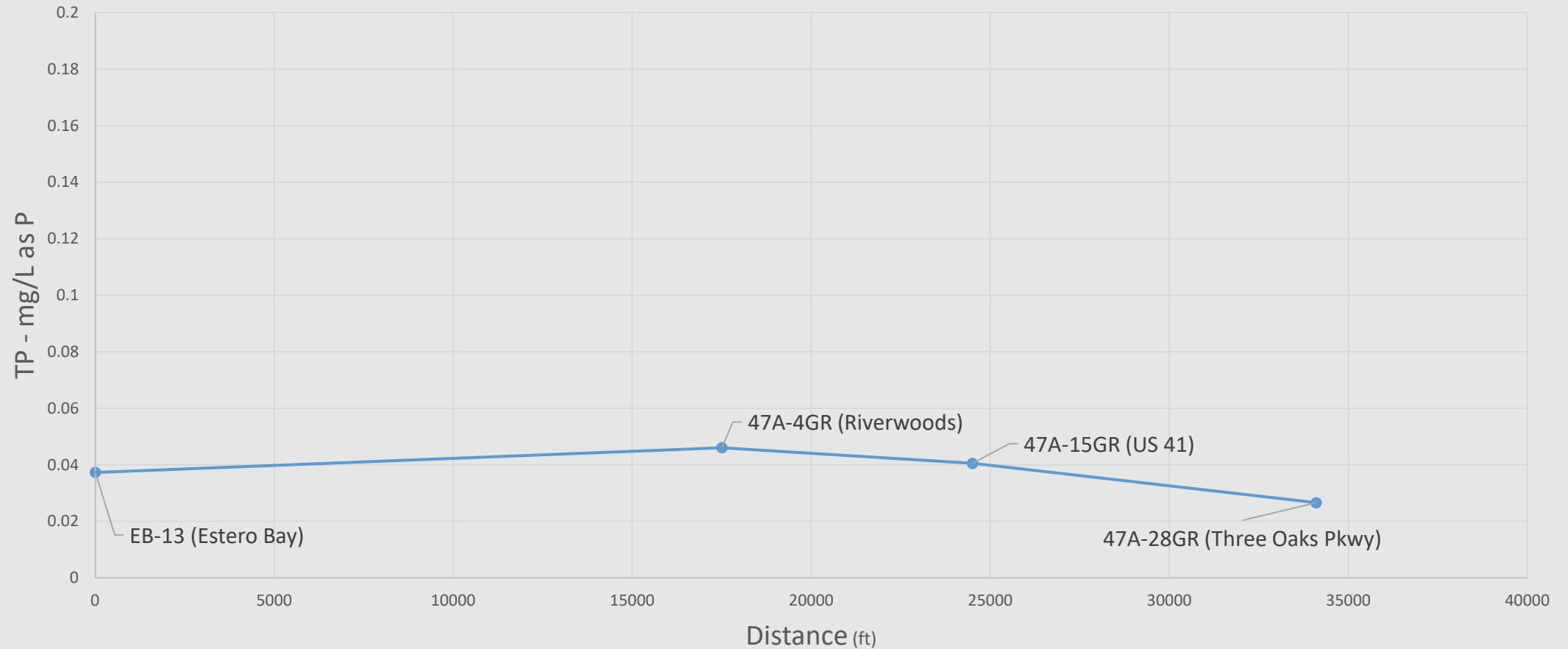
Estero River - Total Phosphorus (TP) Geometric Mean Concentration
