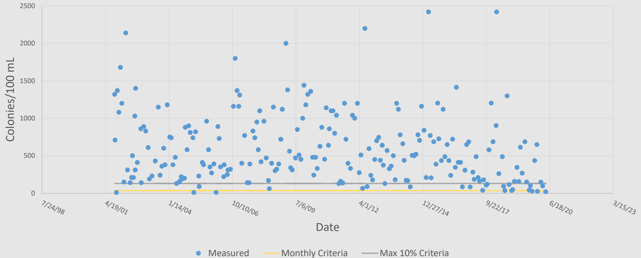
Estero River at US-41 (47A-15GR) Enterococci Bacteria
