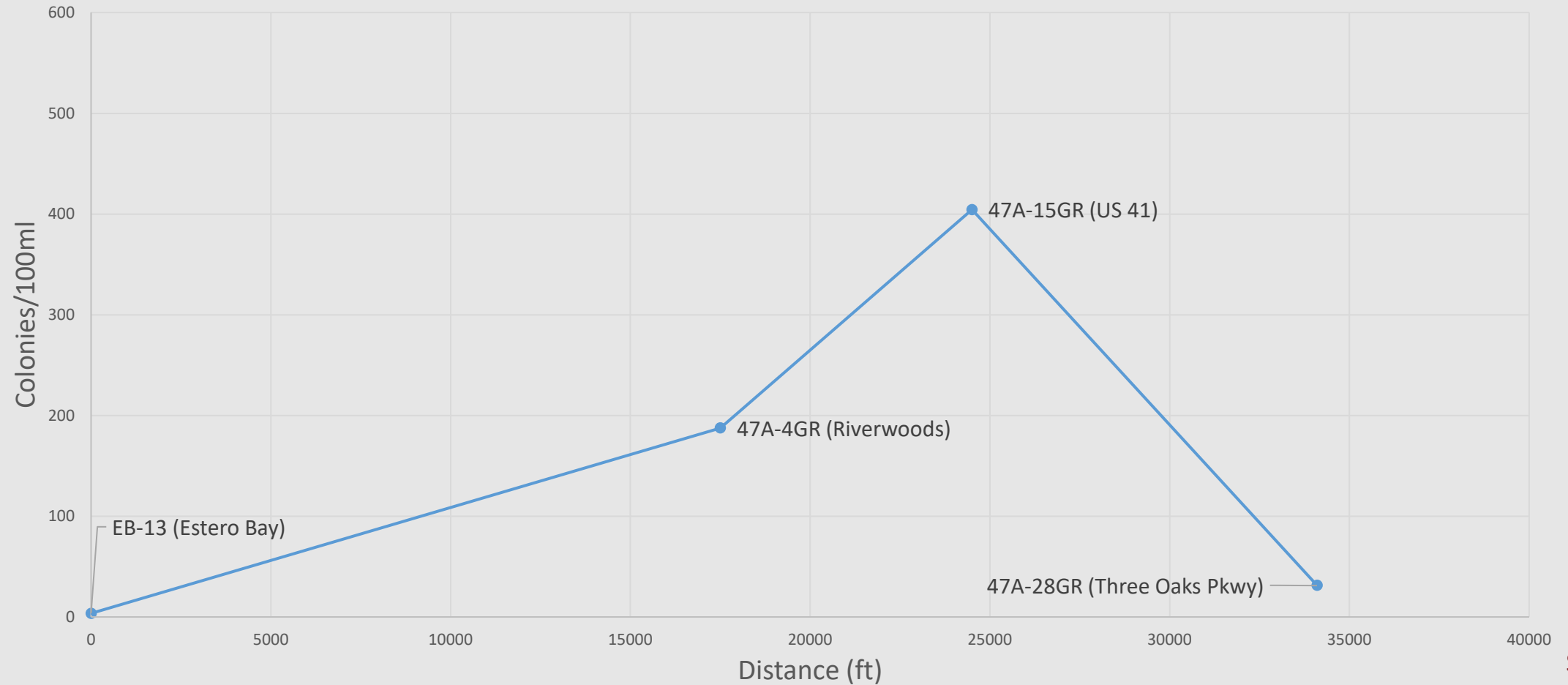
Estero River - Enterococci Bacteria Geometric Mean Colonies
