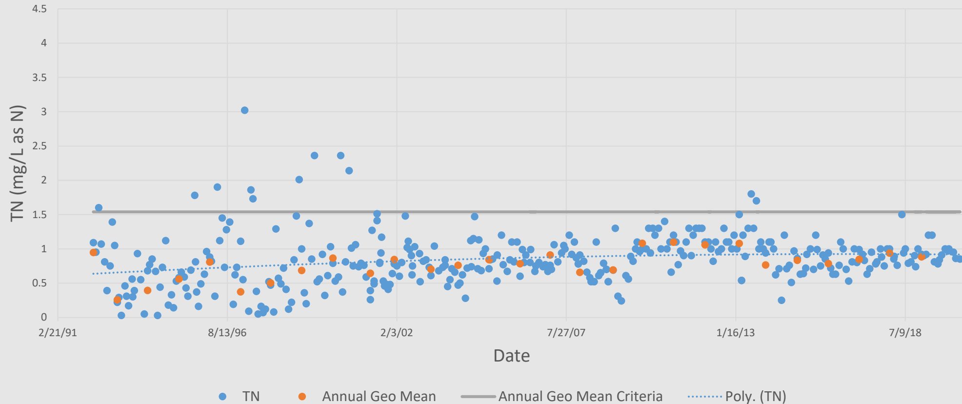
Estero River at US-41 (47A-15GR) Total Nitrogen
