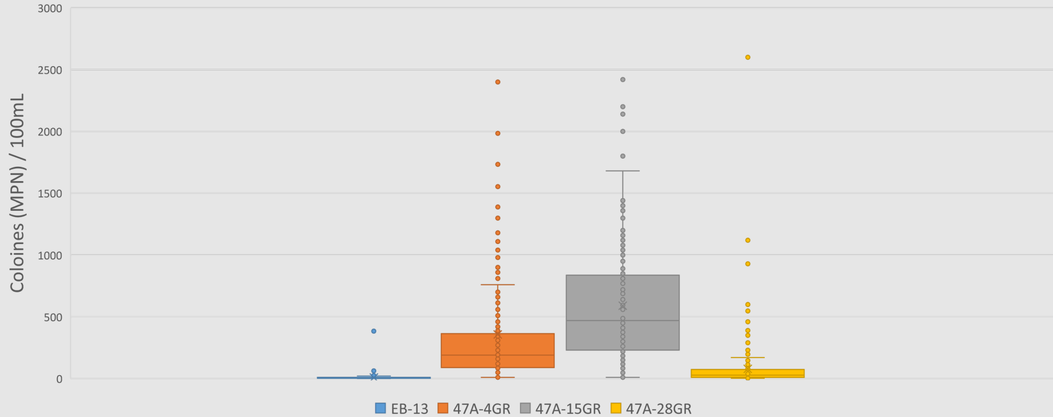
Estero River Enterococci Bacteria (2001-2020)
