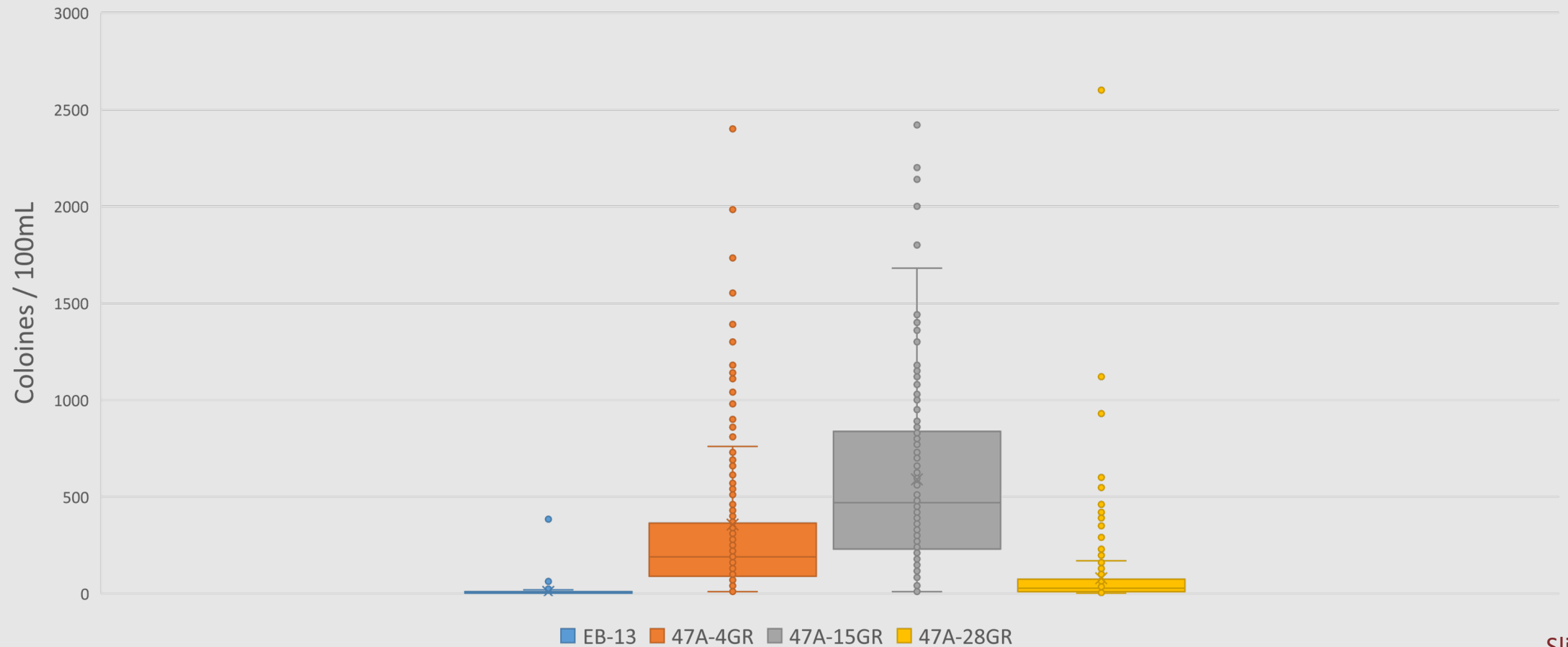
Estero River E. Coli (2001-2020)
