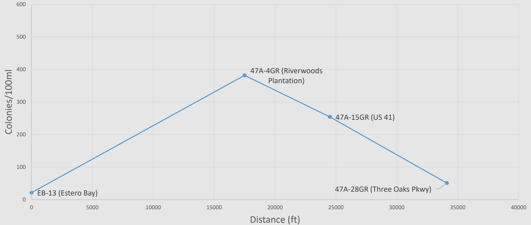
Estero River - E. Coli Geometric Mean Colonies
