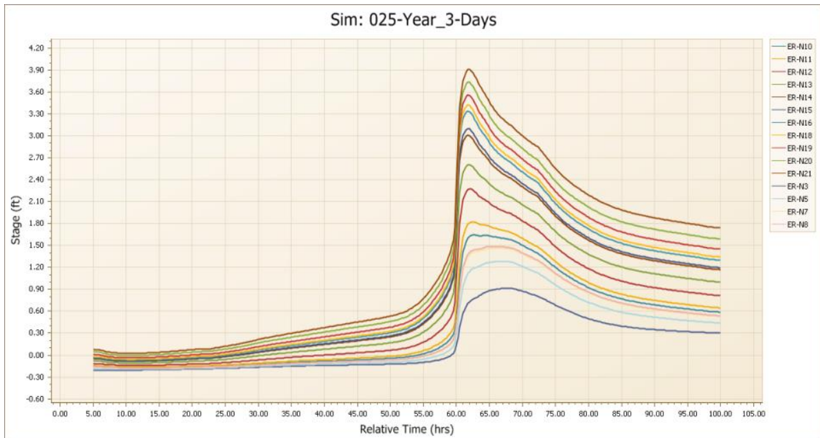
Figure 3-44: Estero River Section 1 - 25-Year, 3-Day Stage Time Series
